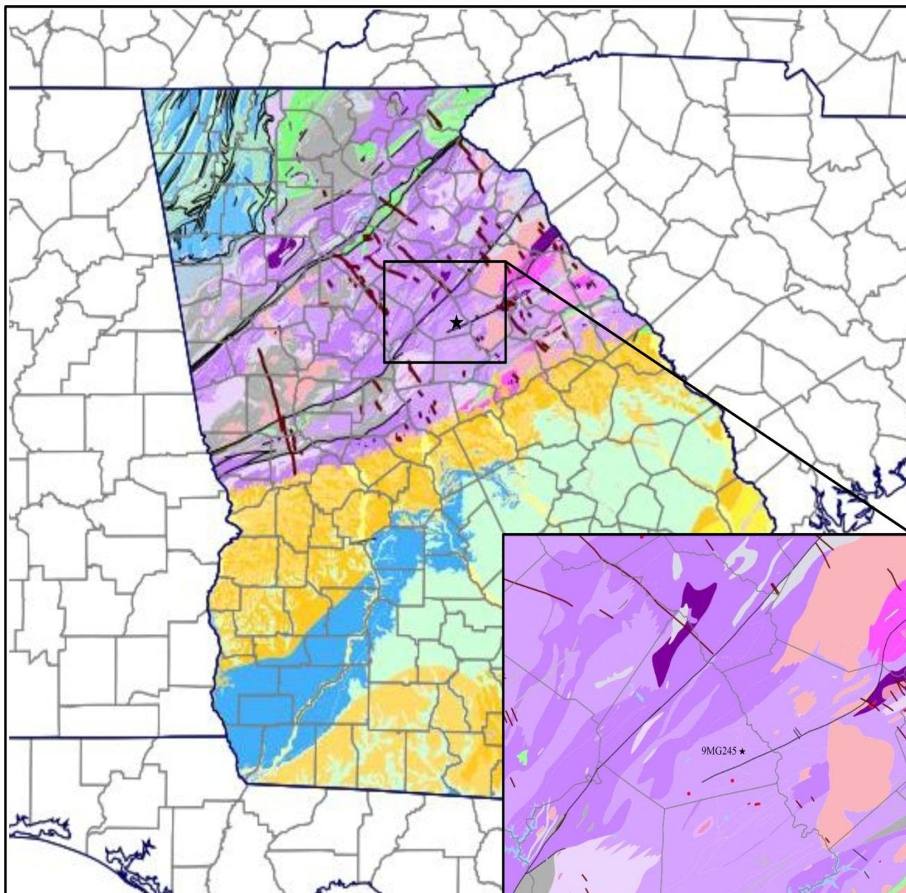
Figure 5. Geologic formations of Morgan County. Georgia geology map and data from USGS Georgia geology website. http://mrdata.usgs.gov/sgmc/ga.html
